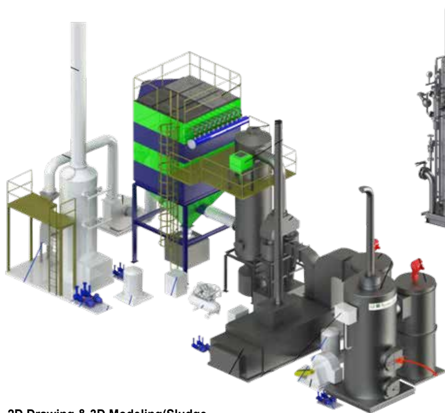
2D Drawing & 3D Modeling(Sludge incinerator Dry, Wet type)
